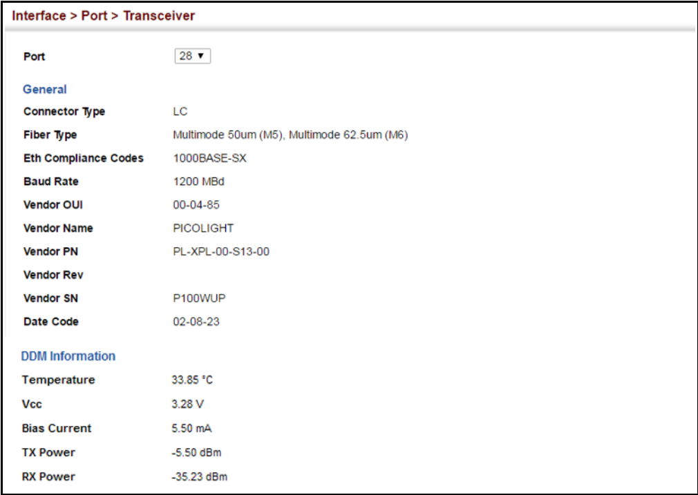
Figure 43: Displaying Transceiver Data
