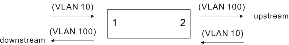
Figure 106: Configuring VLAN Translation
