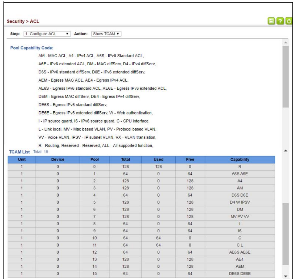
Figure 193: Showing TCAM Utilization
