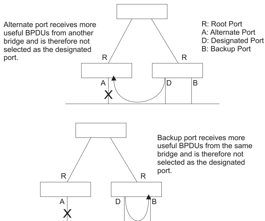
Figure 118: STA Port Roles
